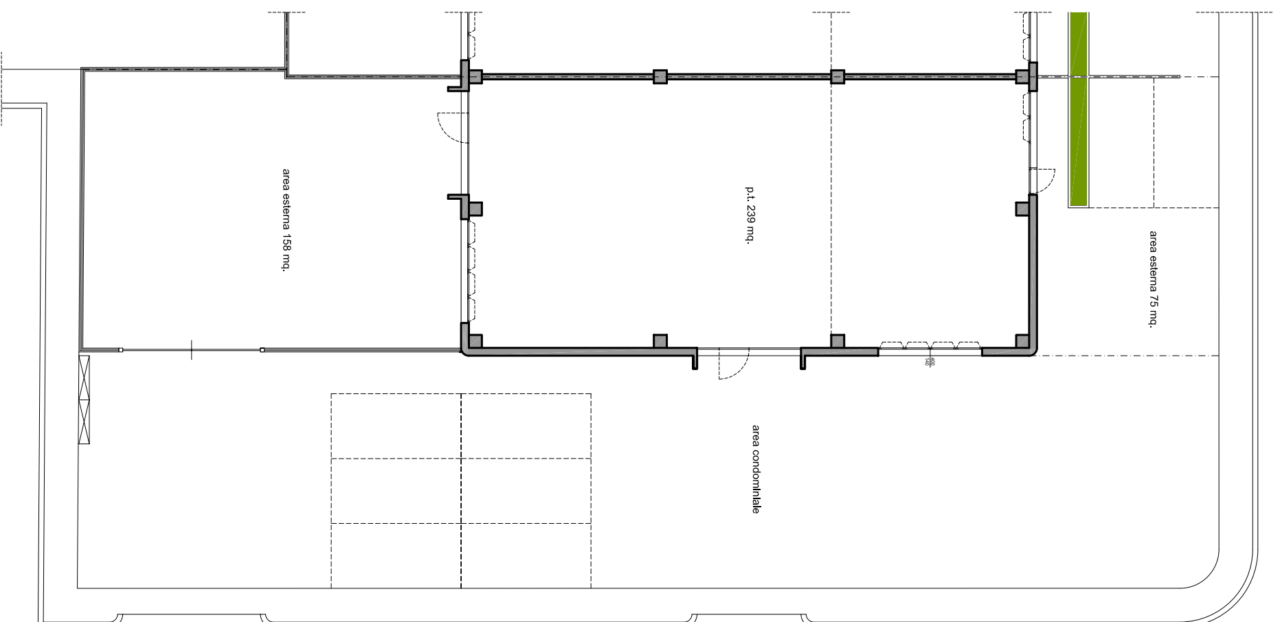
PIANO TERRA
